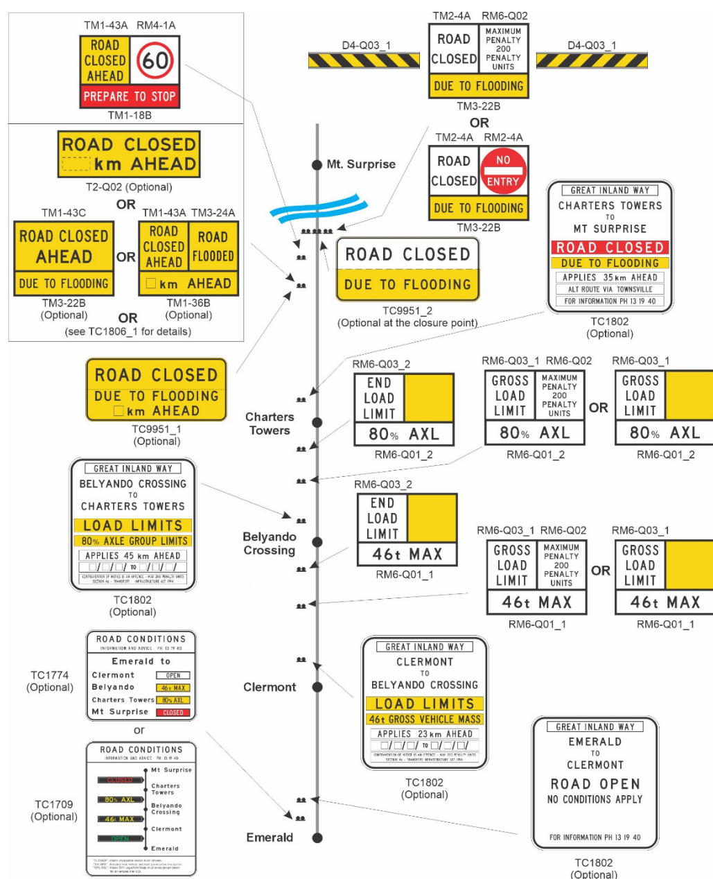
Figure A.6.3 – Example sign layout for a typical route with various restrictions and a closure due to flooding
