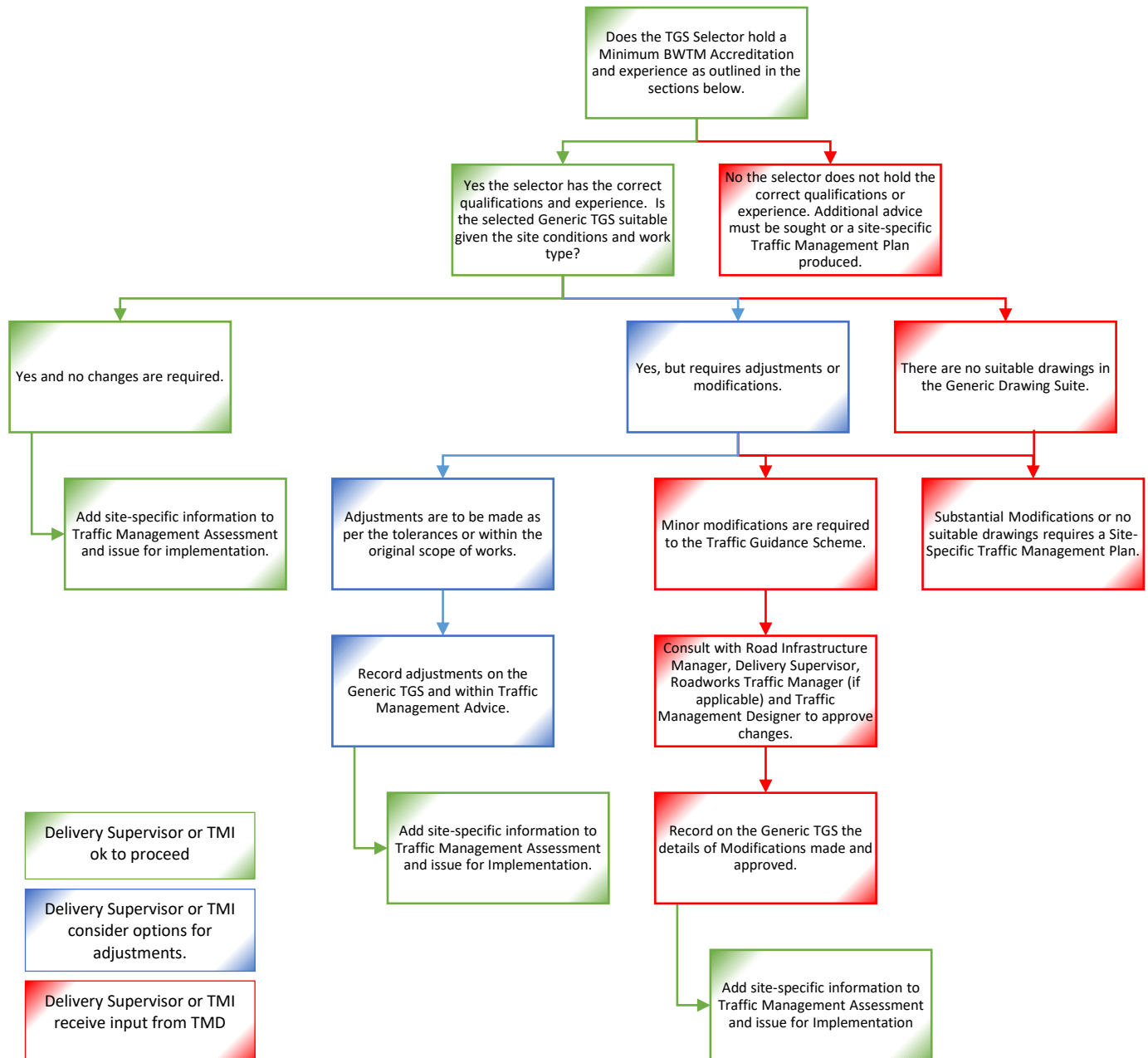
Figure 5: Flow Chart to Select Applicable Traffic Guidance Scheme – AGTTM Part 8 Figure 3.1
