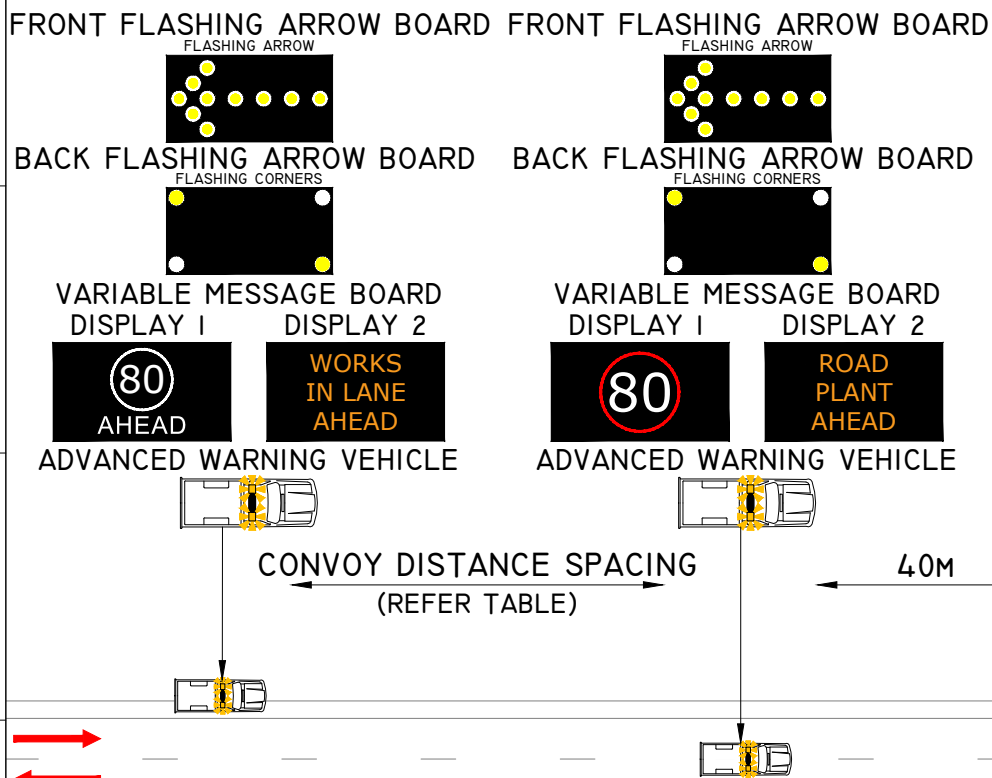
CLASS 2 MOBILE SCENARIO VEHICLES TRAVELLING GREATER THAN 20km/h BELOW THE SPEED LIMIT (NO WORKERS ON FOOT)
