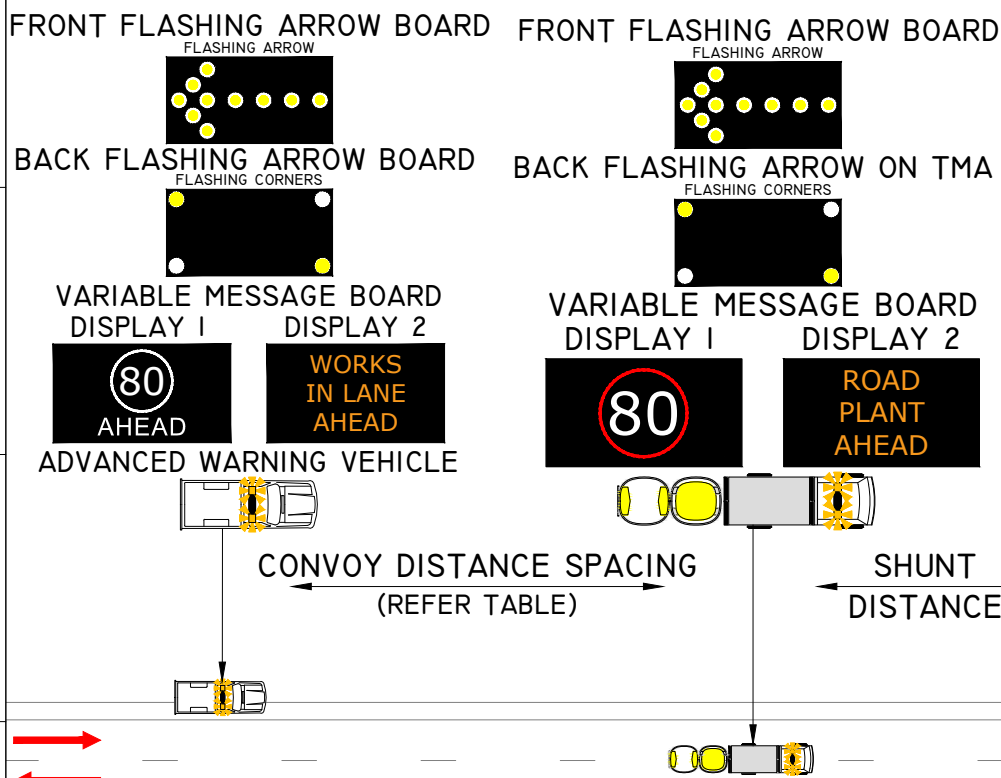
CLASS 2 MOBILE SCENARIO VEHICLES TRAVELLING GREATER THAN 20KM/H BELOW THE SPEED LIMIT (NO WORKERS ON FOOT) TRUCK MOUNTED ATTENUATOR.
