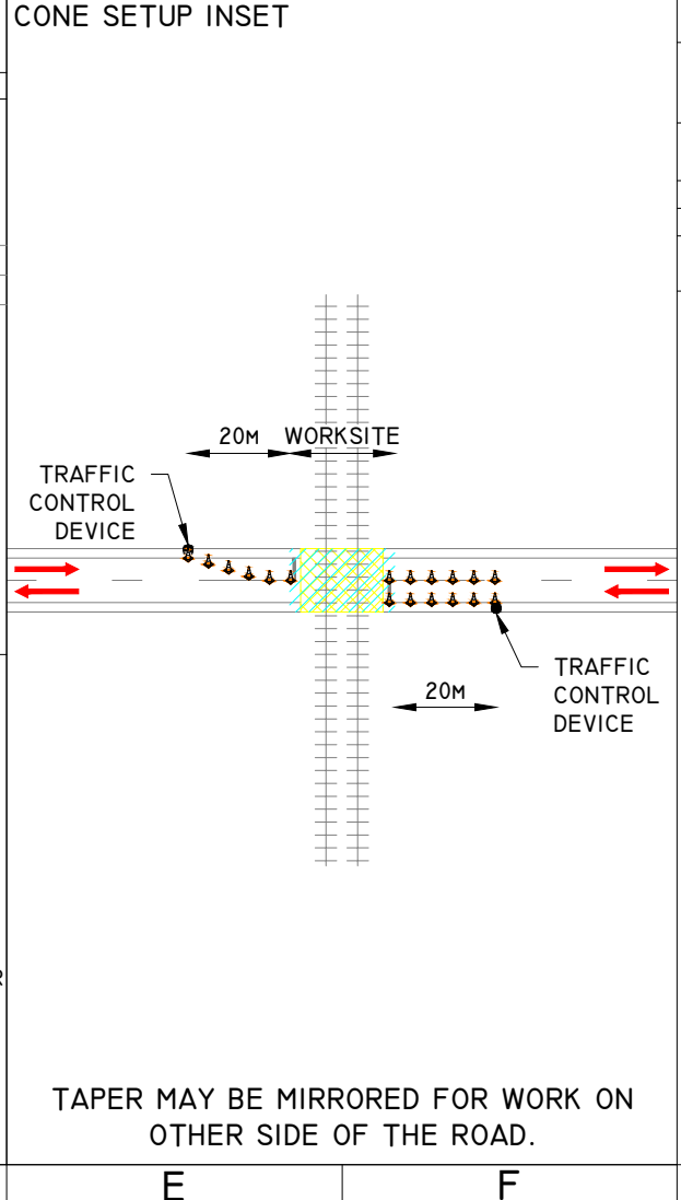
SCENARIO 1: EXISTING 70-110km/h (60km/h TEMPORARY ZONE)
