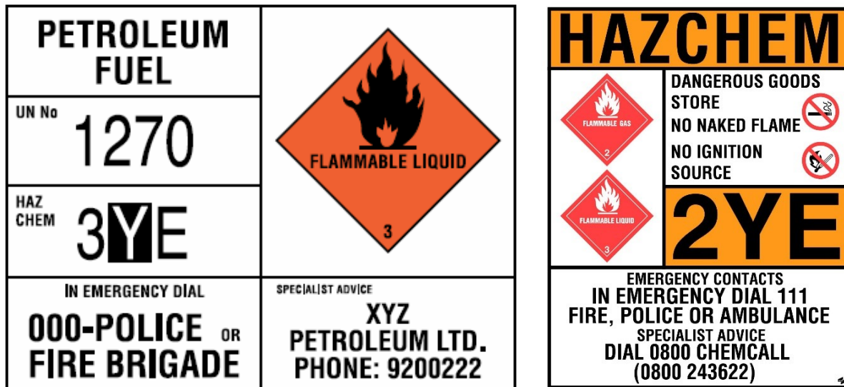
Figure 2.12: Example emergency information to displayed on all hazardous or explosive loads
