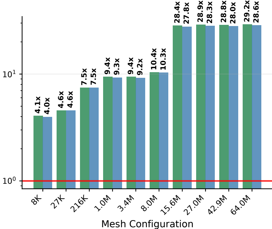
Speedup vs A100 (Legacy)
