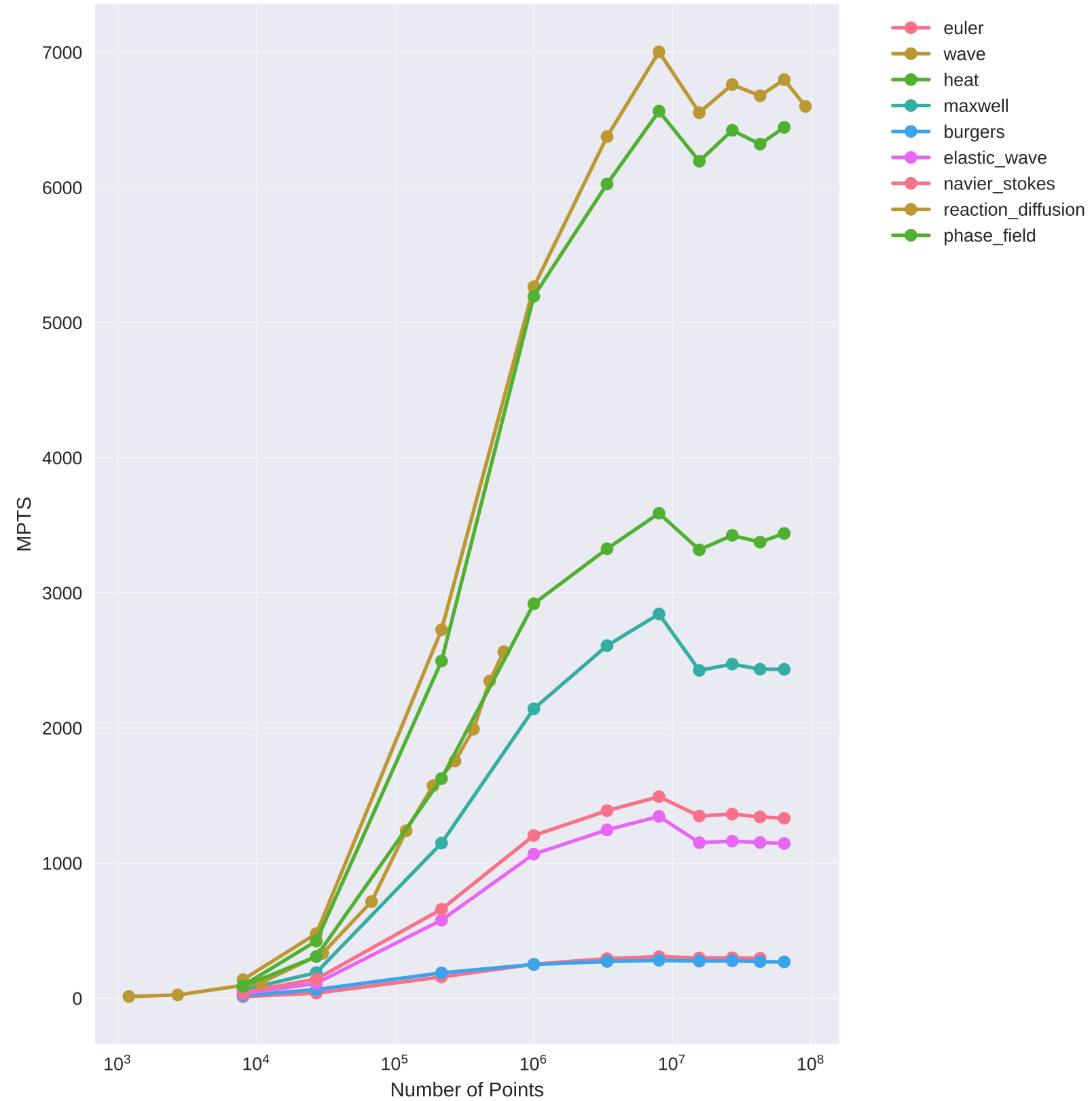
Performance Scaling with Mesh Size
