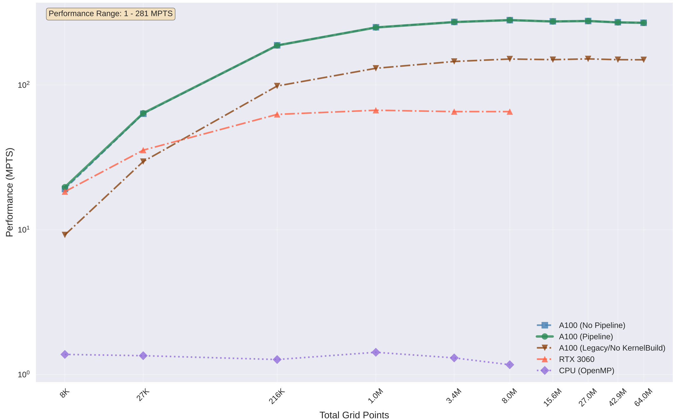
Hardware Performance Comparison: Burgers Equation
