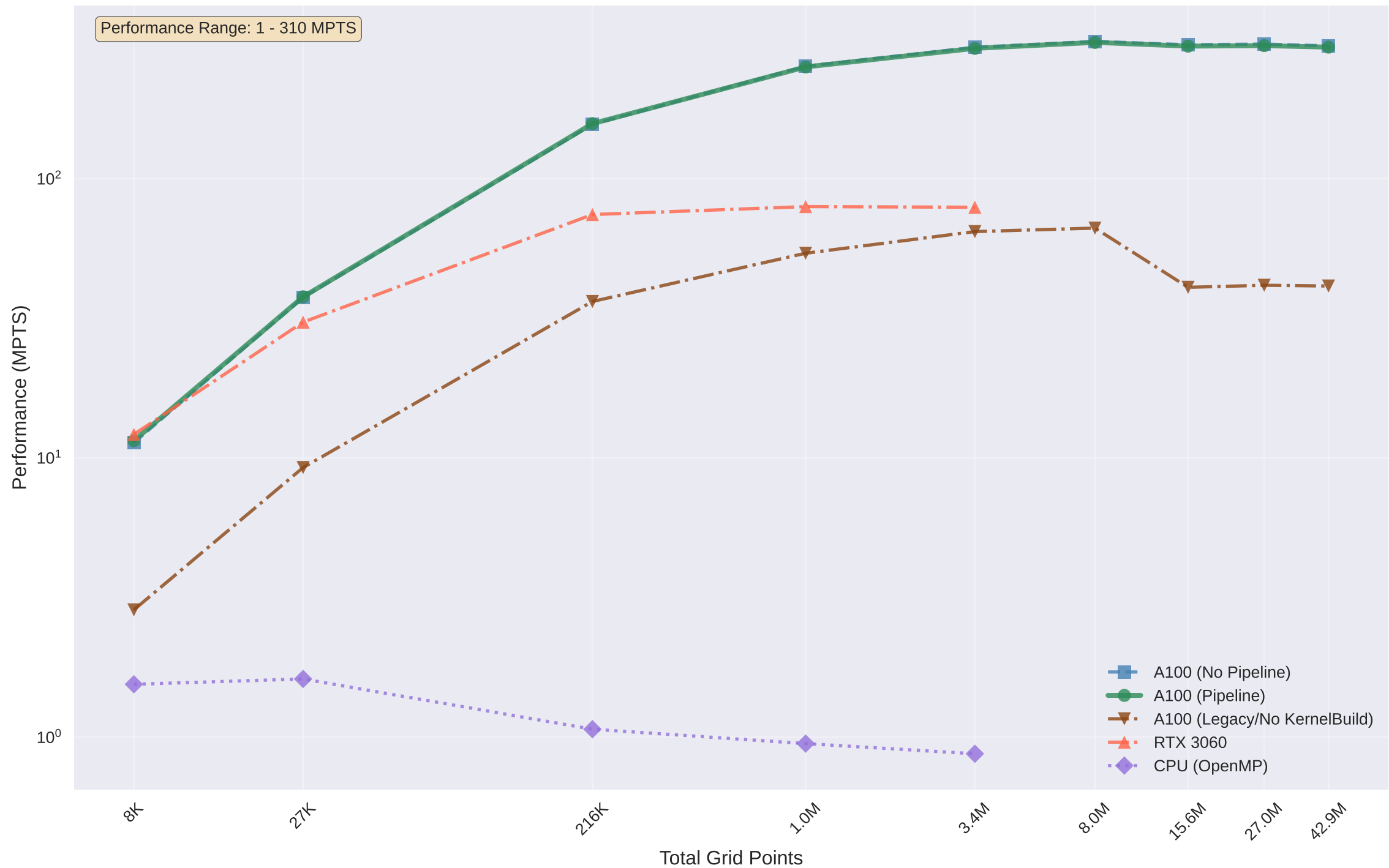
Hardware Performance Comparison: Euler Equation
