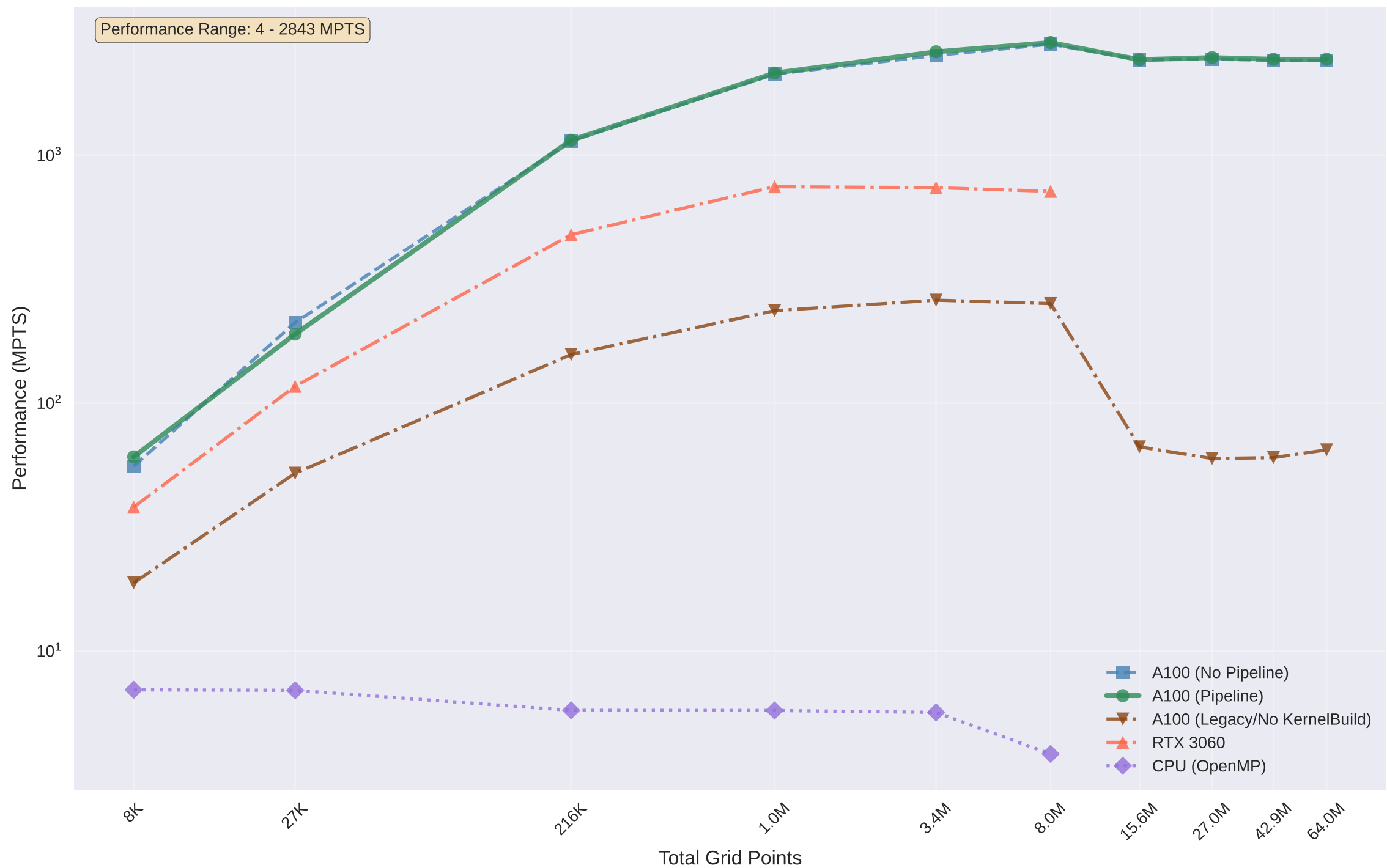
Hardware Performance Comparison: Maxwell Equation
