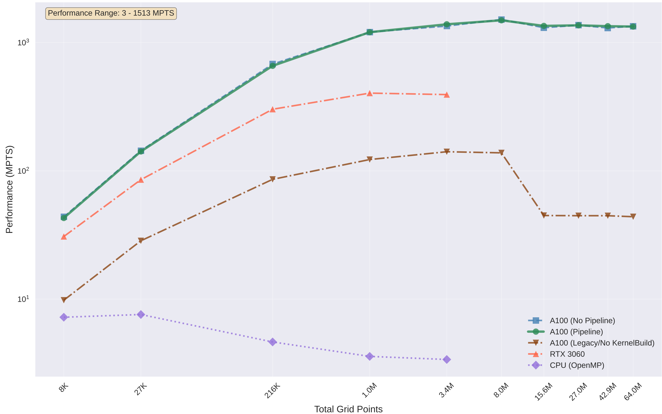
Hardware Performance Comparison: Navier Equation
