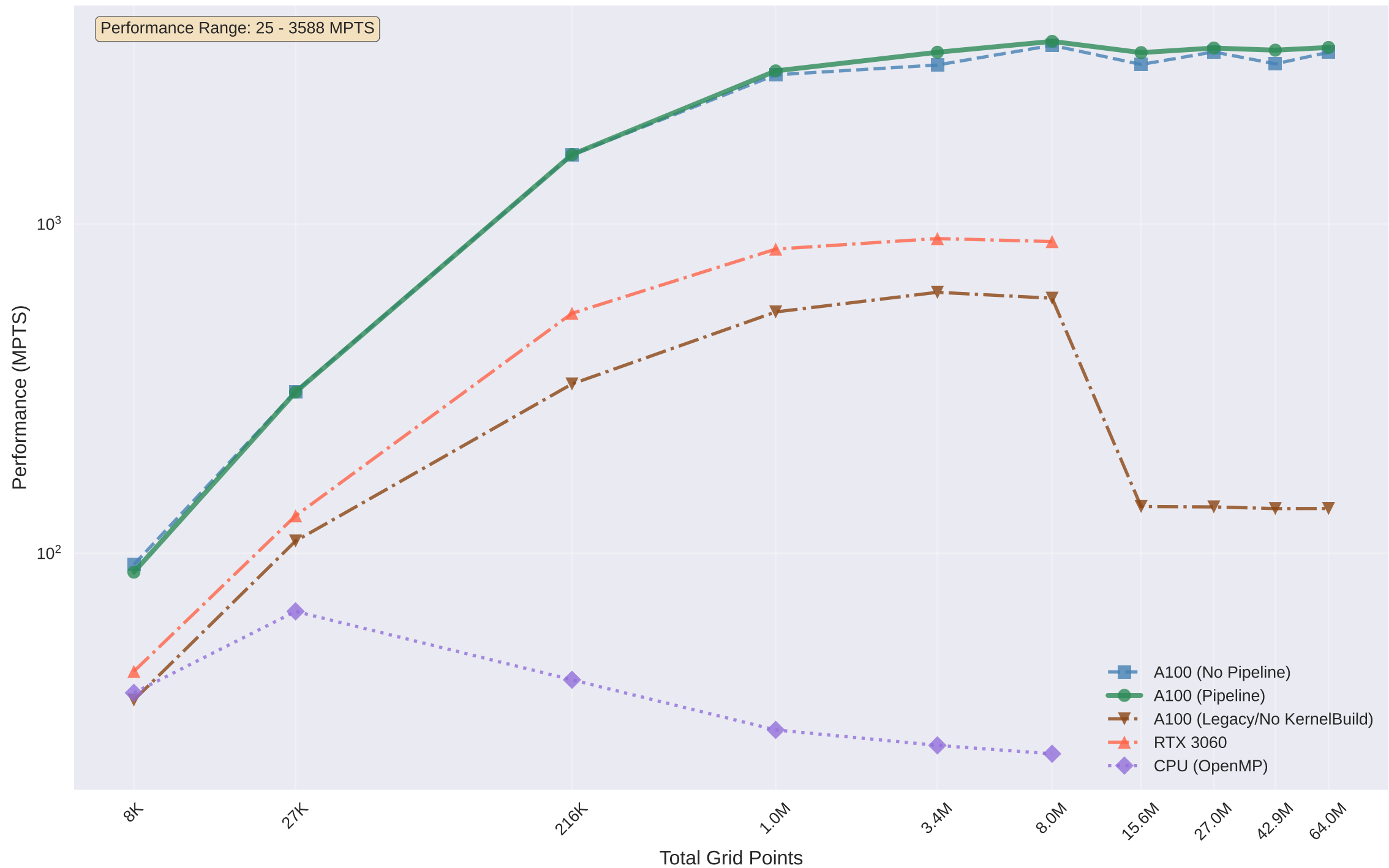
Hardware Performance Comparison: Phase Equation
