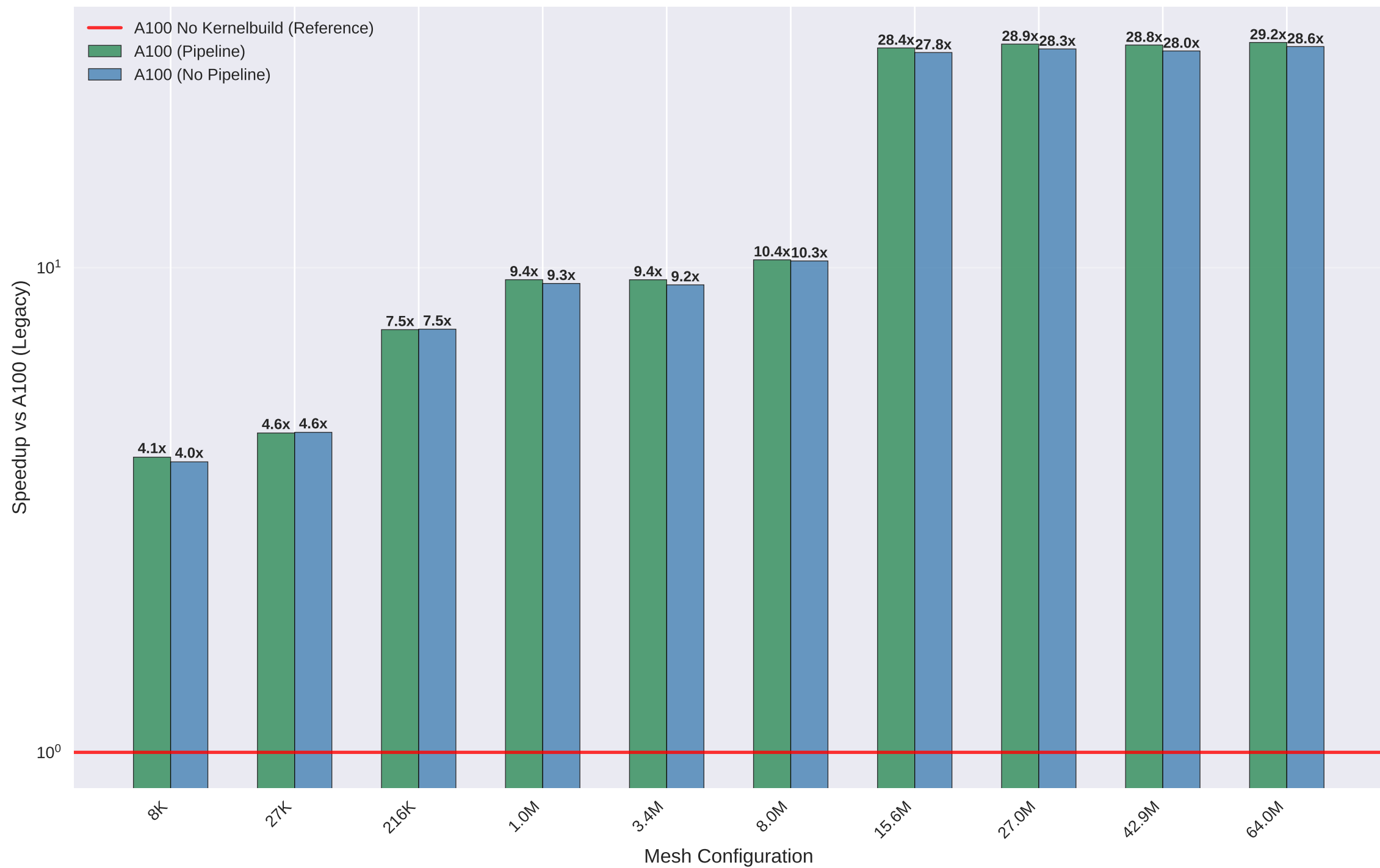
Speedup Scaling vs A100 (Legacy): Elastic Equation
