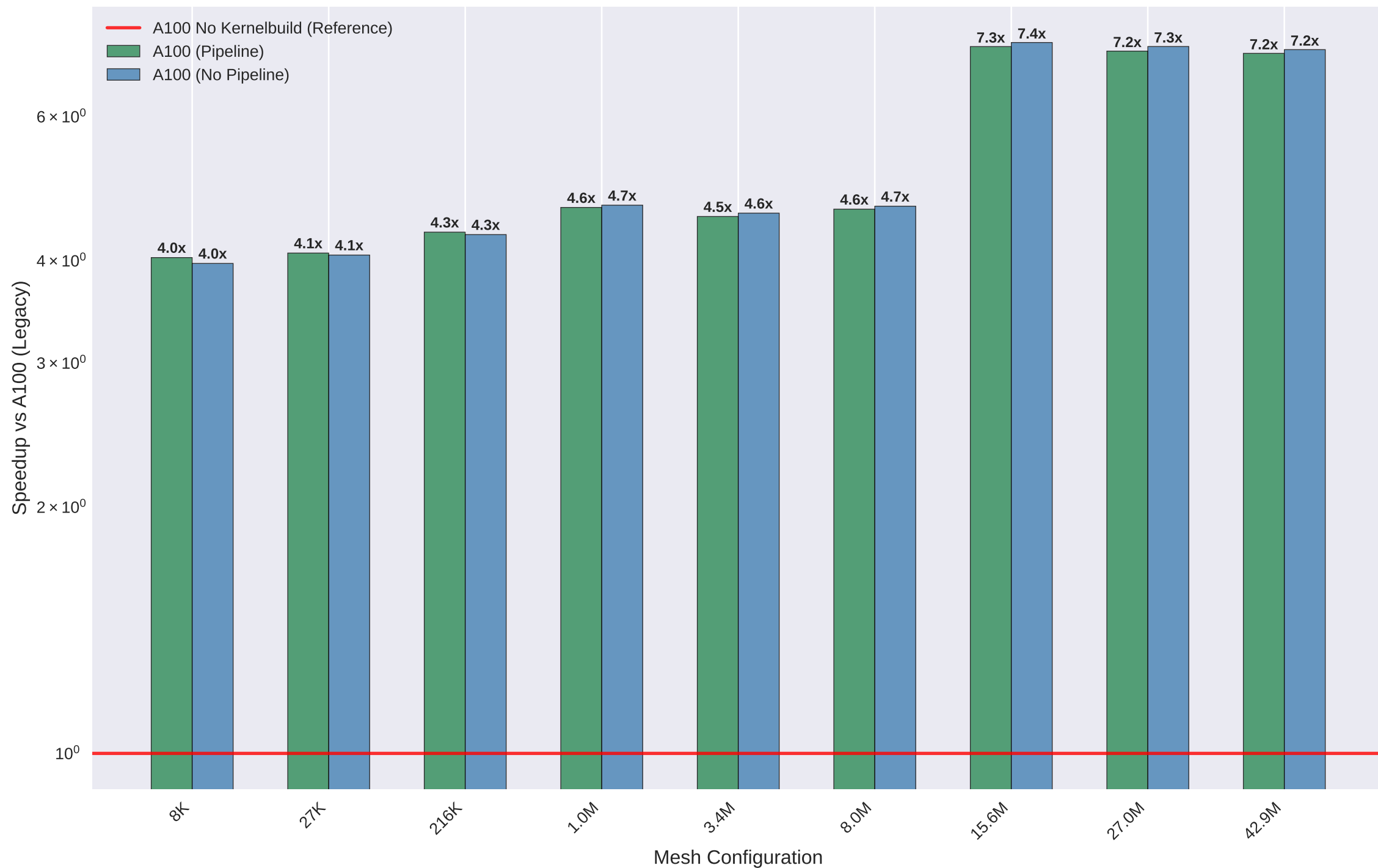
Speedup Scaling vs A100 (Legacy): Euler Equation
