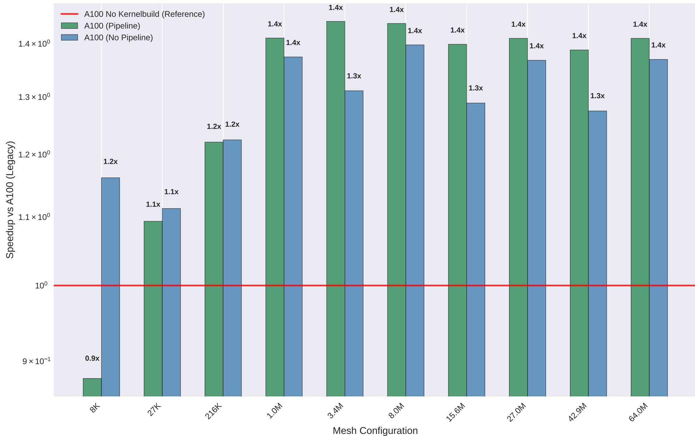
Speedup Scaling vs A100 (Legacy): Heat Equation
