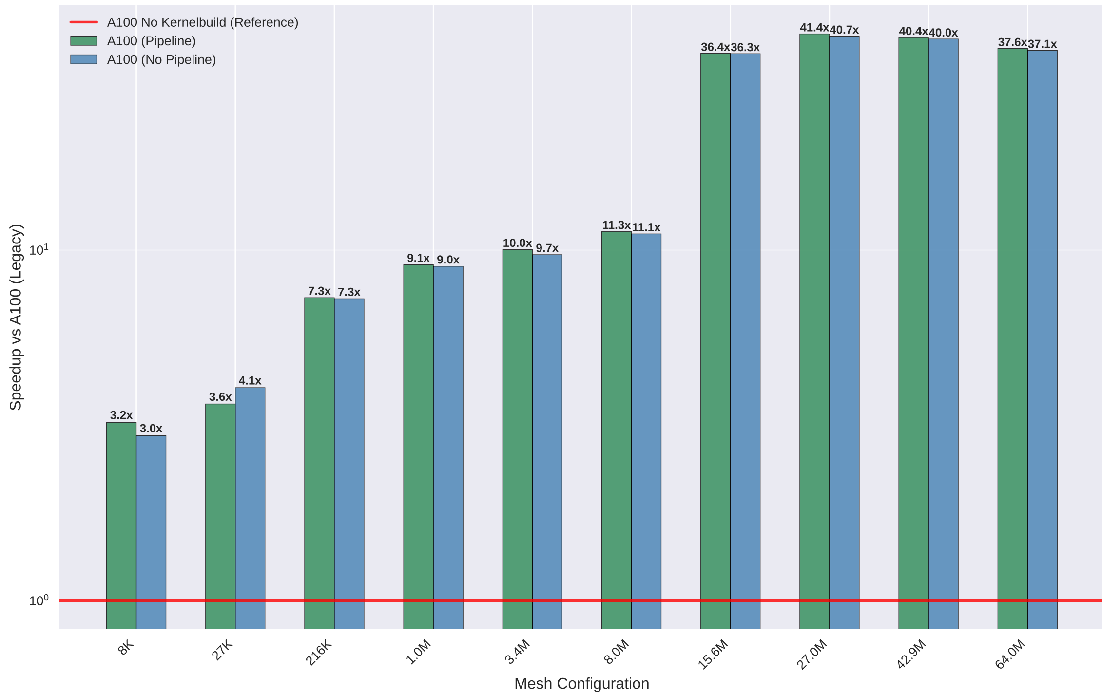
Speedup Scaling vs A100 (Legacy): Maxwell Equation
