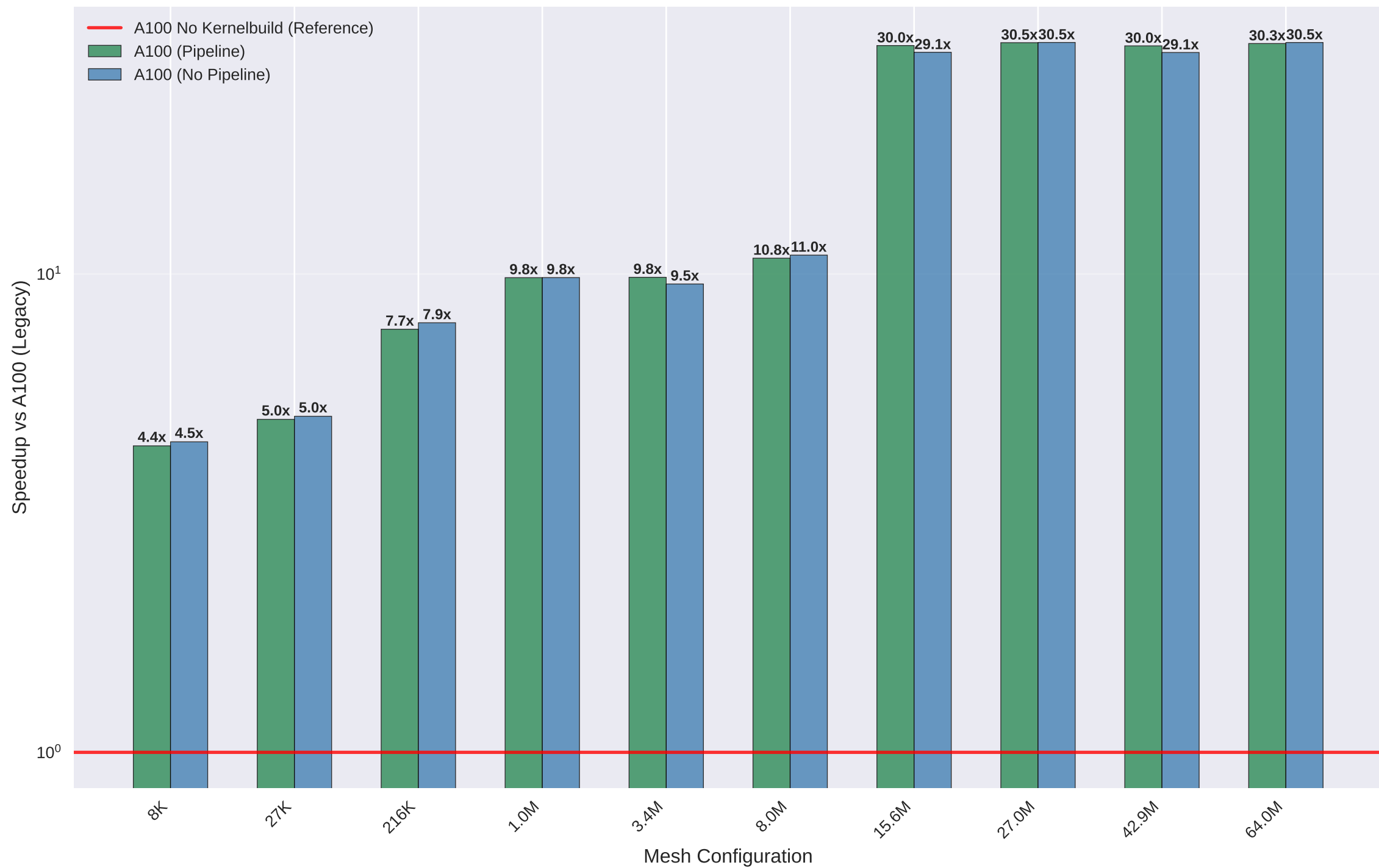
Speedup Scaling vs A100 (Legacy): Navier Equation
