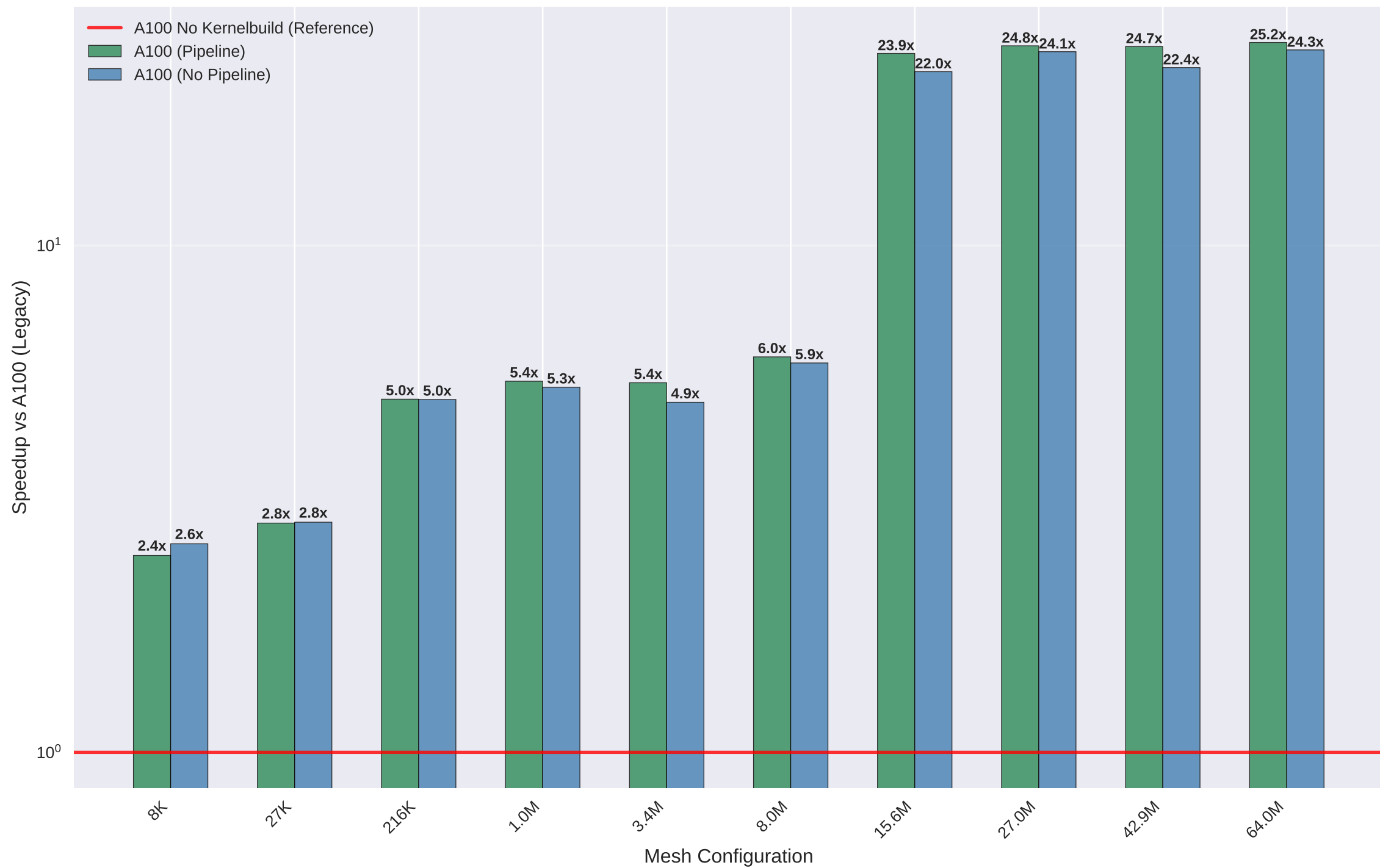
Speedup Scaling vs A100 (Legacy): Phase Equation
