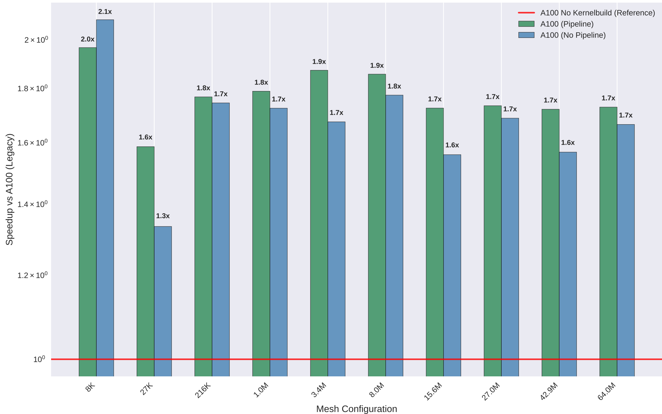
Speedup Scaling vs A100 (Legacy): Wave Equation
