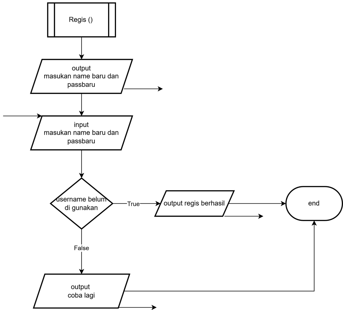
Gambar Flowchart 1.3 (fungsi regis)
