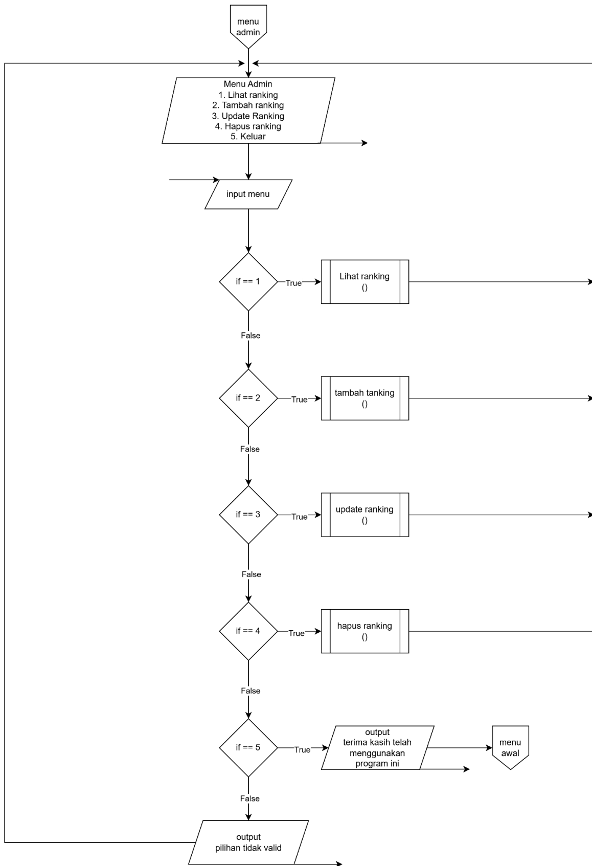
Gambar Flowchart 1.4 (menu admin, bagian admin)
