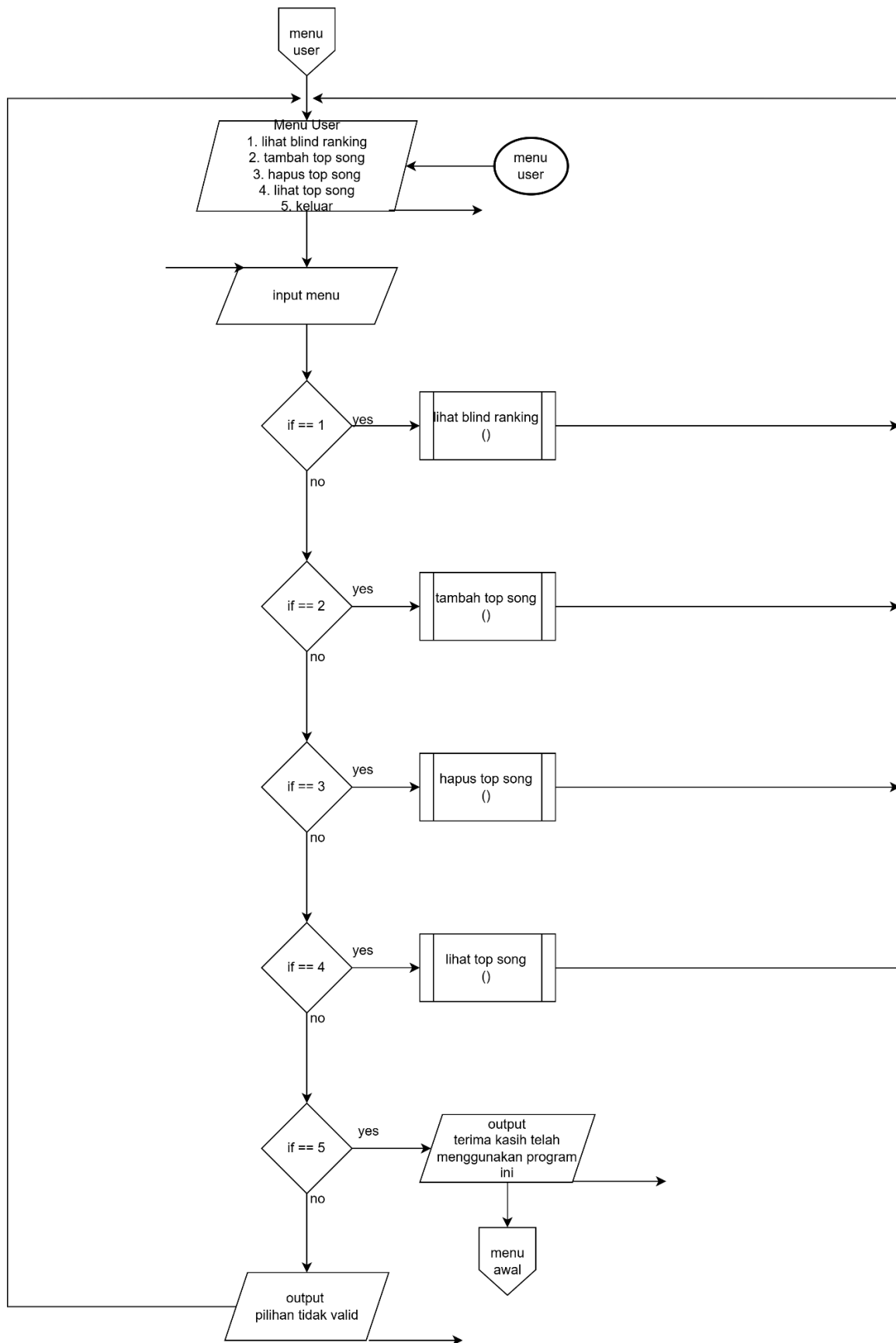
Gambar Flowchart 1.5 (Menu User, bagian user)
