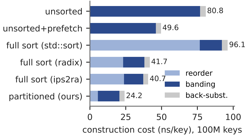
Figure 2: Construction cost by phase, 100M keys. The partition pass replaces the sort at 4\times lower reorder cost while banding stays within 13% of banding-after-full-sort.
