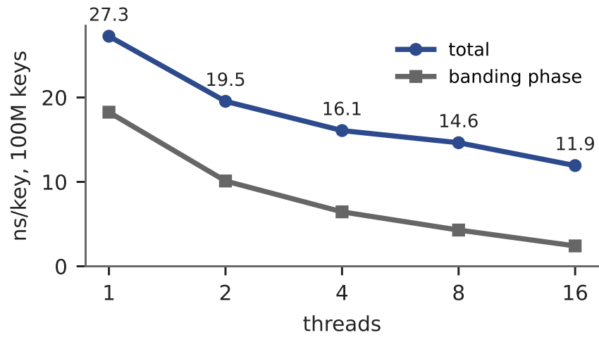
Figure 2: Slot-range parallel construction, 100M keys; every point bit-identical to the sequential build.
