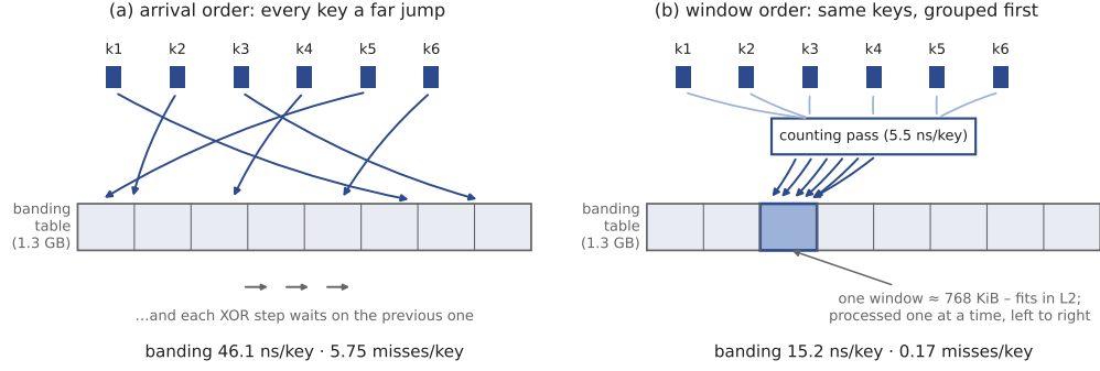
Figure 1: Effect of insertion order on banding. (a) In arrival order, every key starts its elimination at a random position in a table far larger than the L2 cache, and the steps within each insertion form a dependent chain no prefetcher can run ahead of. (b) A counting pass assigns keys to table windows, and a scatter pass groups them by window; banding then works inside one cache-resident window at a time. Binary fuse filters apply the same remedy to their counter scatter via a segment sort (§2). Numbers: 100M keys, means of 3 runs.
