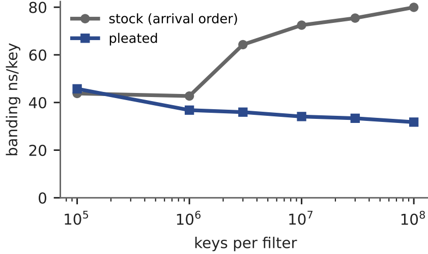
Figure 4: RocksDB Standard128 ribbon banding-phase cost vs. filter size. Pleated banding cost does not rise (cache-resident per window); stock banding degrades as the table outgrows cache. Measured false-positive rates match stock to six digits at every point.
