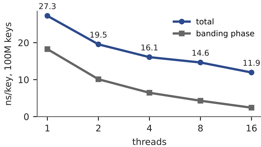
Figure 3: Slot-range parallel construction, 100M keys; every point bit-identical to the sequential build.
