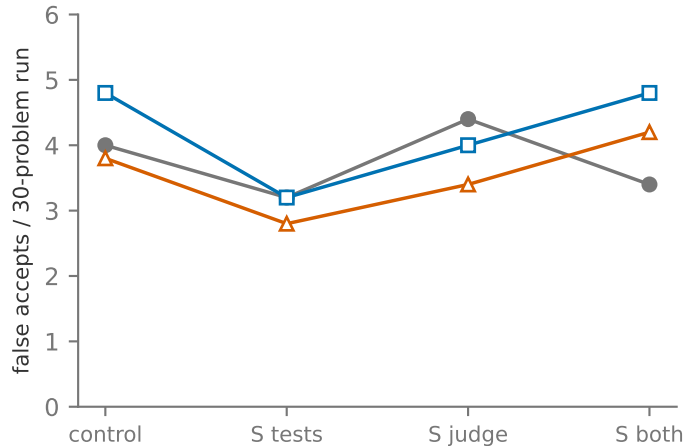
HumanEval+
