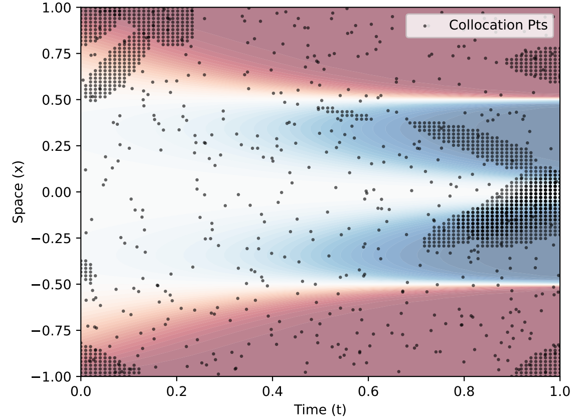
Temporal Variance (TVAR) Final MAE: 0.30767
