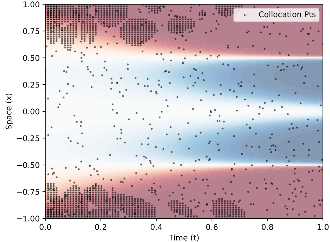
Residual Refinement (RAR) Final MAE: 0.56458
