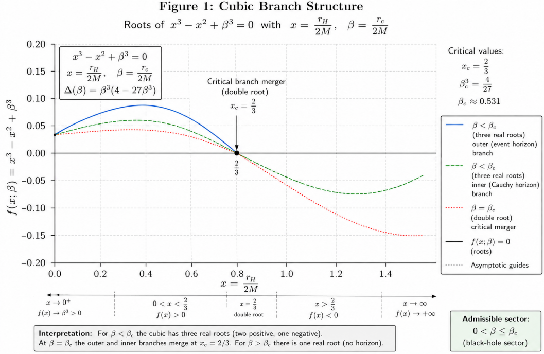
Figure 1: Cubic branch structure associated with the TIG2 horizon relation x^3 - x^2 + \beta^3 = 0 . The figure illustrates the admissible horizon branches, the critical branch-merger point x_c = 2/3 , and the discriminant-controlled transition separating admissible and non-admissible sectors.
