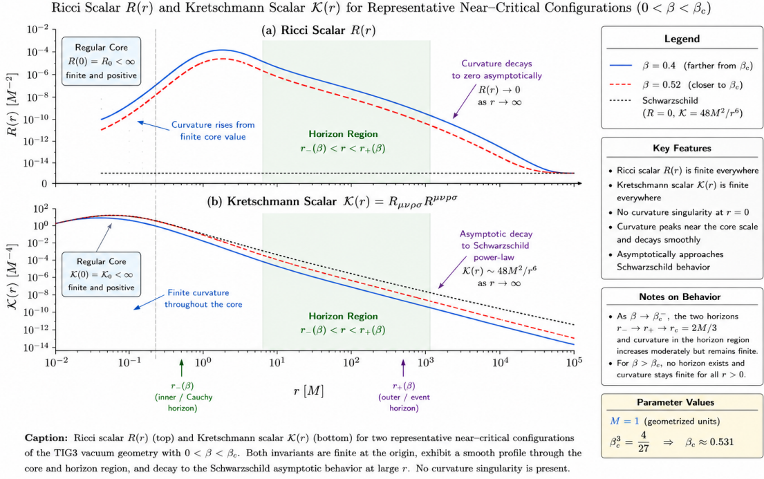
Figure 4: Curvature Invariants in TIG3 Vacuum Geometry
