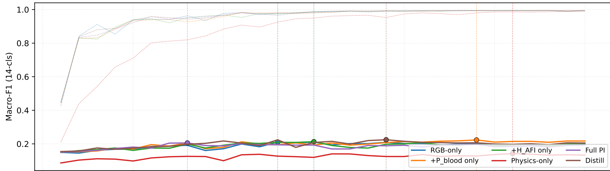
Training curves: val (solid) vs train (dotted). Markers = trainer's chosen best epoch (val macro-F1, 14-cls).
