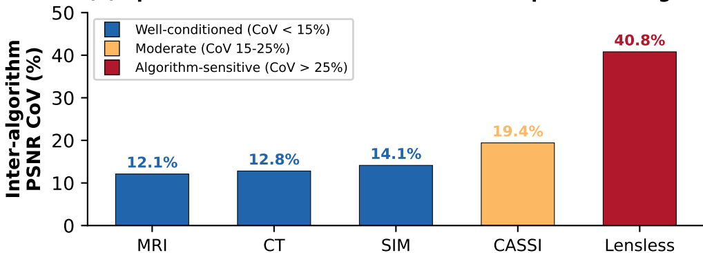
(a) Specification dominance: CoV across 5 published algorithms
