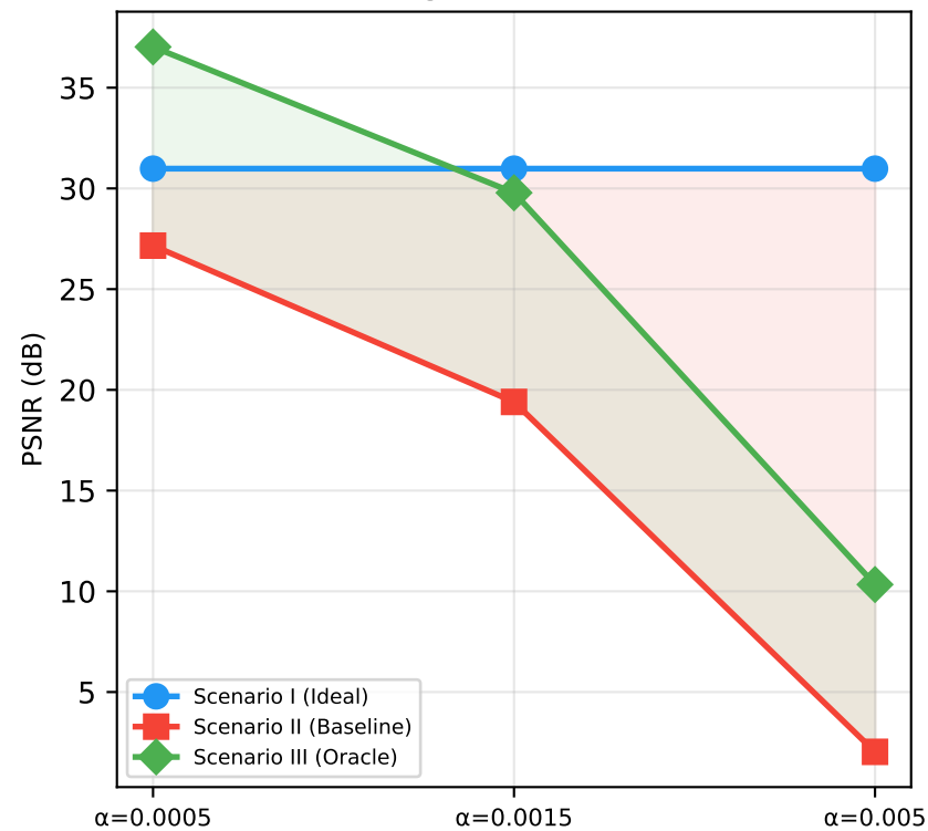
SPC — HATNet (gain drift \alpha )
