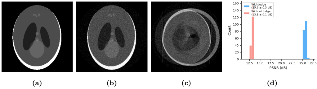
Figure 4. CT reconstruction comparison (modified Shepp–Logan phantom, 128 projections, Poisson noise, n = 200 ). (a) Ground truth. (b) Framework with Judge ( \in \mathfrak{S} verified): correct angular model, Ram-Lak filter, non-negativity enforced. (c) Without Judge: wrong angular range ( 360^\circ assumed instead of 180^\circ ), producing doubled edges and streak artifacts; 5,326 non-negativity violations. (d) PSNR distribution: with Judge 25.6 \pm 0.3 dB vs. without Judge 13.1 \pm 0.1 dB ( n = 200 , p < 10^{-30} , Wilcoxon).
