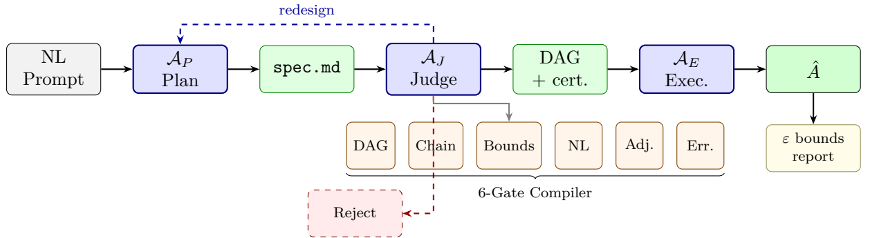
Figure 3. Specification-driven design pipeline. A natural-language prompt is the sole user input. \mathcal{A}_P generates a spec.md ; \mathcal{A}_J validates it via a 6-gate compiler (Gates 1–3 from FPB compiler [3]; Gates 4–6 new to this work; mapping to Theorem 2: DAG \rightarrow \varepsilon_{\text{spec}} , Chain \rightarrow \varepsilon_{\text{trans}} , Bounds \rightarrow complexity, NL \rightarrow \varepsilon_{\text{param}} , Adj. \rightarrow consistency, Err. \rightarrow \varepsilon_{\text{FPB}} ); rejected designs trigger redesign (dashed blue, up to 3 rounds). \mathcal{A}_E executes reconstruction and outputs \hat{A} with an explicit \varepsilon -bound report. See Figure 4 for per-modality error breakdown.
