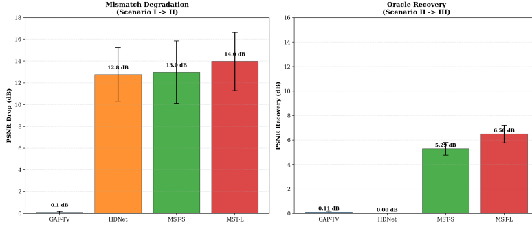
Fig. 2: CASSI mismatch degradation (left, \Delta_{\text{deg}} ) and oracle recovery (right, \Delta_{\text{rec}} ) per method under 5-parameter mismatch. HDNet shows zero recovery due to its mask-oblivious architecture. MST-L achieves the highest recovery (+6.50 dB), though the moderate recovery ratio (46.5%) reflects the difficulty of correcting dispersion mismatch with current fixed-step architectures.
