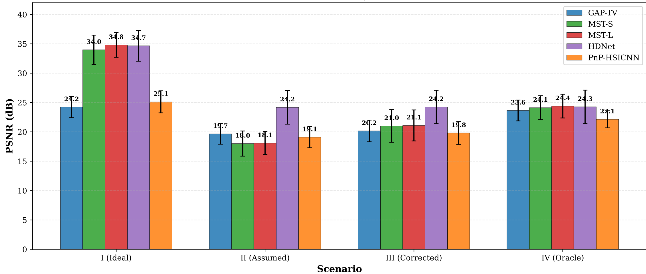
CASSI Reconstruction Quality Across 4 Scenarios
