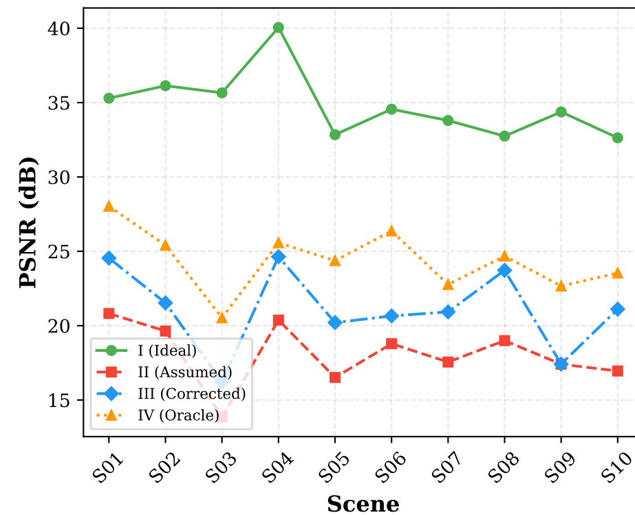
MST-L
