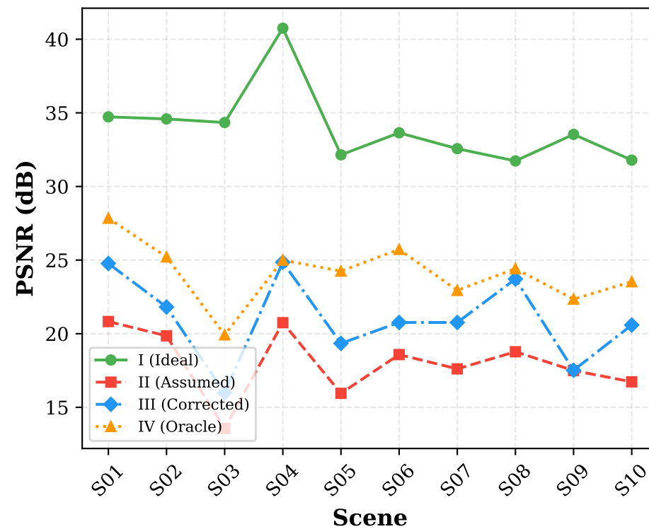
PnP-HSICNN
