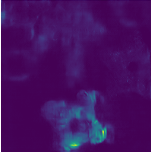
MST-S (mismatched)
