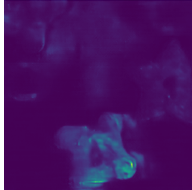
MST-L (mismatched)
