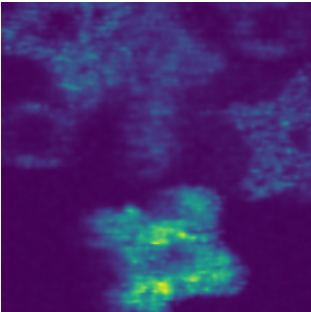
GAP-TV (mismatched)
