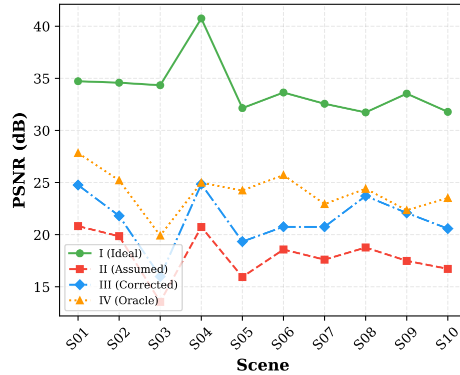
PnP-HSICNN
