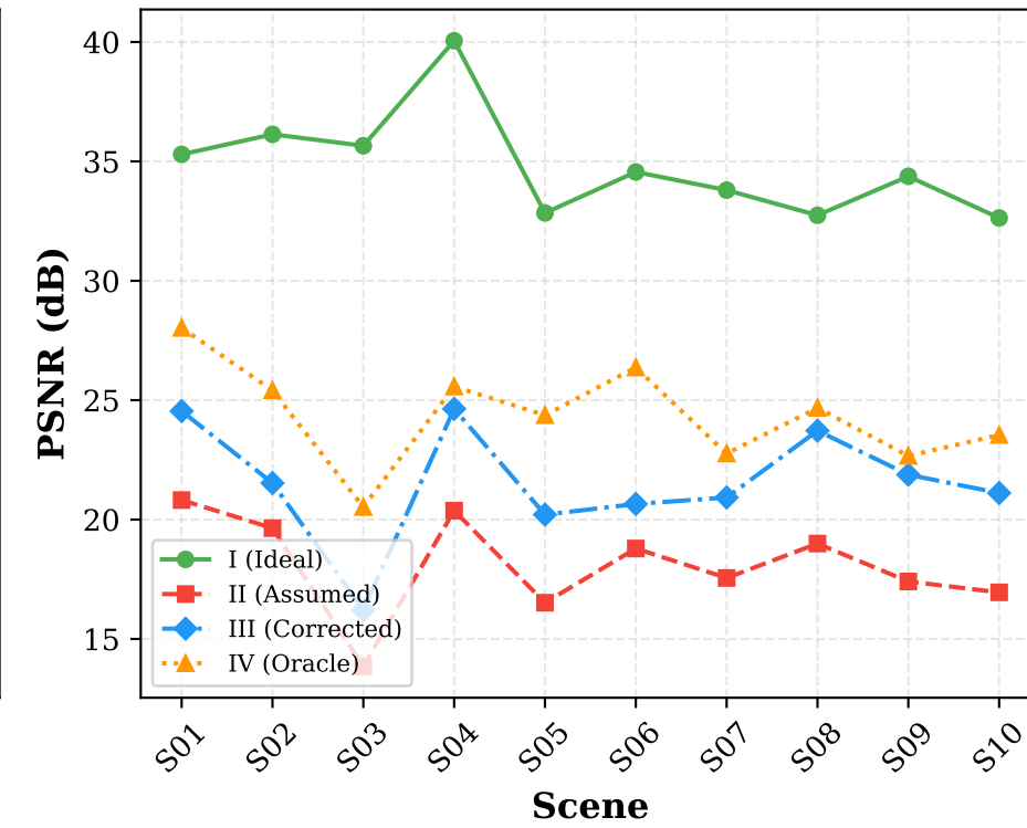
MST-L
