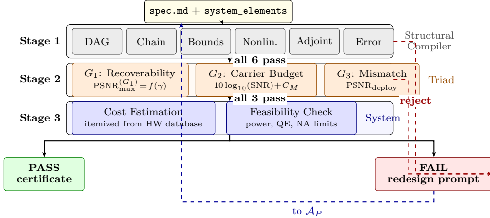
Figure 6. Judge Agent validation flow. Stage 1: a 6-gate structural compiler rejects malformed specifications before physics evaluation. Stage 2: three deterministic Triad gates [3] diagnose recoverability ( G_1 ), carrier budget ( G_2 ), and operator mismatch ( G_3 ), each with a quantitative margin in dB. Stage 3: hardware cost estimation and physical feasibility assessment. Failure at any stage produces a redesign prompt fed back to the Plan Agent.
