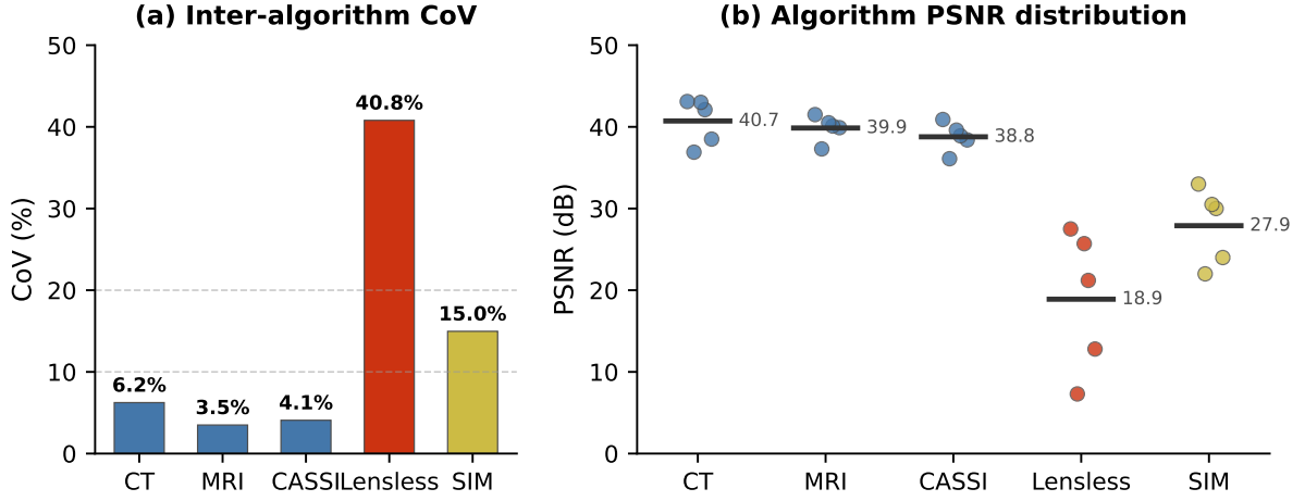
Figure 7. Extended Data Figure 2: Algorithm sensitivity by modality. (a) Inter-algorithm PSNR Coefficient of Variation (CoV) for the top-5 published reconstruction algorithms per modality. Well-conditioned systems (blue, \text{CoV} \approx 3.5\text{--}6.2\% ) show tight convergence among the top algorithms. SIM shows moderate CoV (15.0%). Ill-conditioned compressive systems (red, \text{CoV} > 40\% ) show a wider spread, indicating greater sensitivity to algorithm selection. (b) Individual algorithm PSNR values (dots) with mean (horizontal bar) for each modality. Data from Extended Data Table 7.
