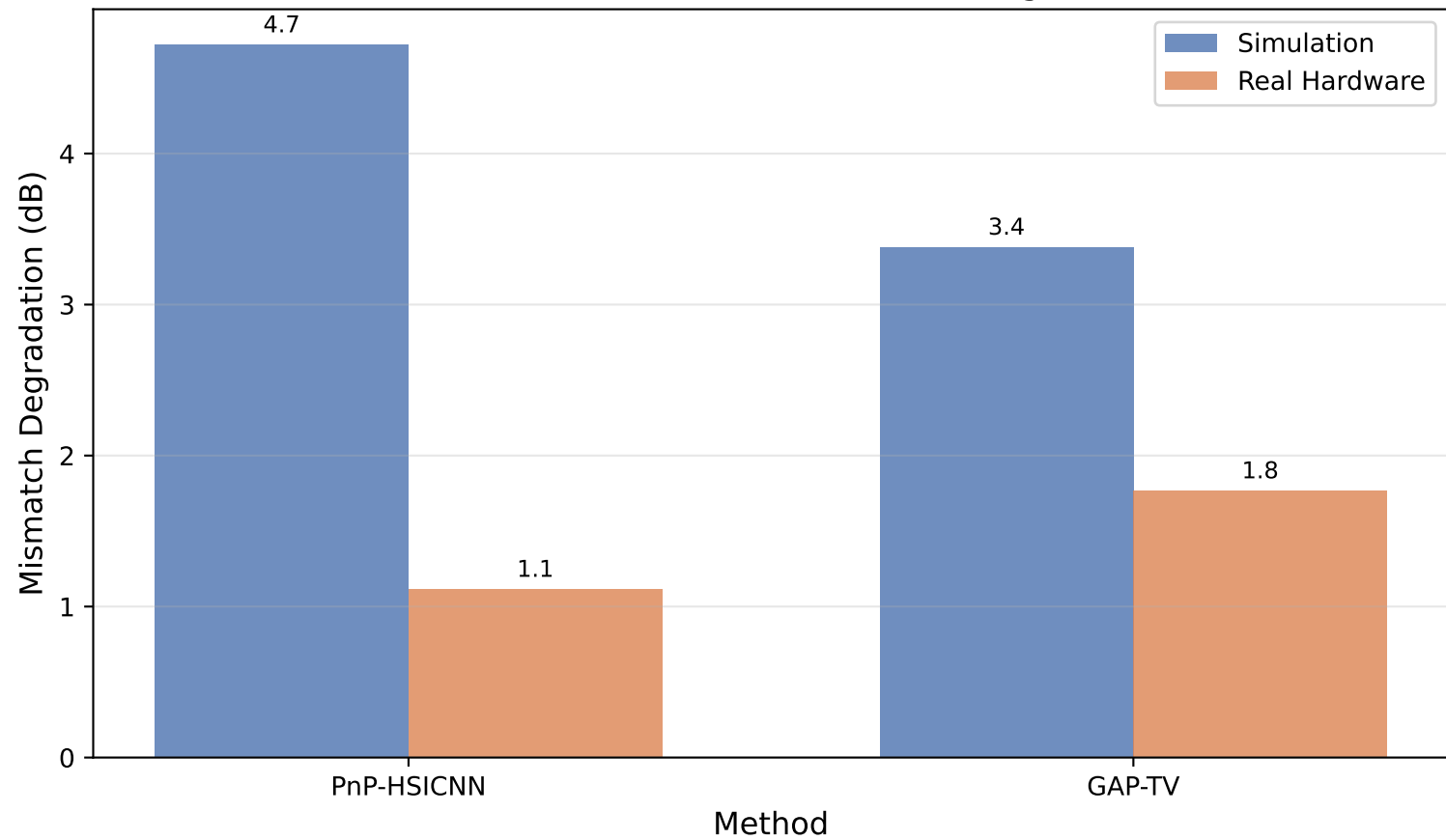
CASSI: Simulation vs Real Hardware Degradation
