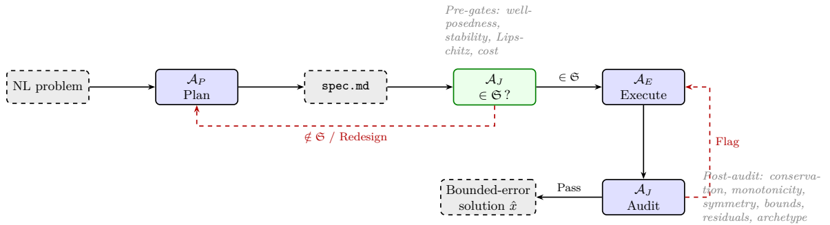
Figure 1. Three-agent pipeline grounded in the simulability class \mathfrak{S} . The Plan Agent translates natural language into a spec.md file (realizing S1). The Judge Agent verifies S2–S4 via 5 pre-execution gates and audits the solution via post-execution quality checks (realizing S4). Rejection triggers redesign (up to 3 rounds) or a certificate that the problem lies outside \mathfrak{S} .
