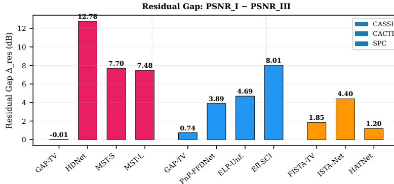
Fig. 5: Residual gap ( \Delta_{\text{res}} = \text{PSNR}_{\text{I}} - \text{PSNR}_{\text{III}} ) per method, grouped by modality. CASSI exhibits the largest residual gaps due to dispersion mismatch that oracle mask correction alone cannot address. CACTI and SPC residual gaps are small, confirming high recoverability of spatial and gain-type mismatches.
