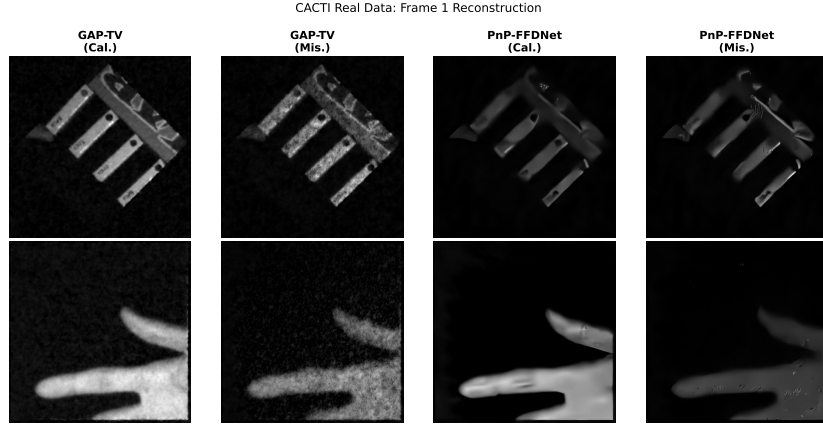
Fig. 2: CACTI real data: calibrated vs. mismatched reconstruction for duomino and hand scenes. Mismatched masks produce temporal ghosting artifacts, mirroring simulation findings.
