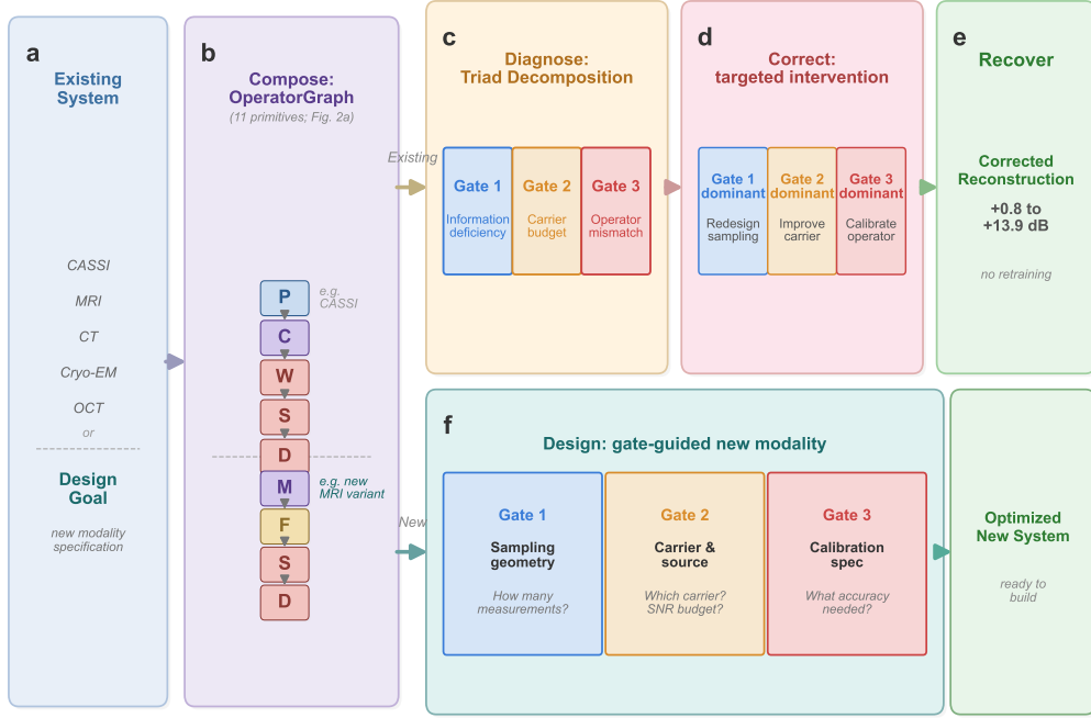
Figure 1: The universal grammar of computational imaging. a , Any computational imaging system—from coded-aperture cameras to cryo-electron microscopes—serves as input. b , The system is composed as a typed directed acyclic graph (DAG) over 11 universal primitives (Figure 2); shown here for CASSI as an example. The grammar enables two workflows. Top (existing instruments) : c , The TRIAD DECOMPOSITION diagnoses the DAG through three independent gates: information deficiency (Gate 1), carrier budget (Gate 2), and operator mismatch (Gate 3). d , Based on the dominant gate, a targeted correction is applied: sampling redesign (Gate 1), source/detector improvement (Gate 2), or operator calibration (Gate 3). e , The existing solver is re-run with the corrected operator, recovering +0.8 to +13.9 dB without retraining. Bottom (new instruments) : f , The same three gates guide the design of a new modality from first principles: Gate 1 determines sampling geometry, Gate 2 guides carrier and source selection, and Gate 3 predicts the calibration accuracy required for a target reconstruction quality. Together, the 11 primitives (alphabet) and 3 gates (rules) form a universal grammar for designing, diagnosing, and correcting any imaging system.
