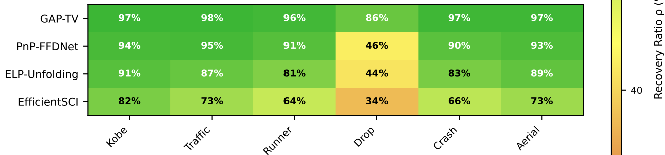
CACTI
