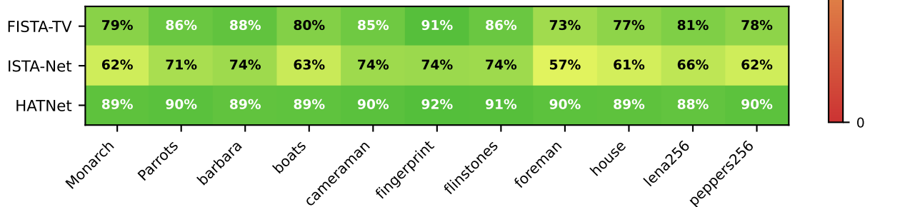
SPC
