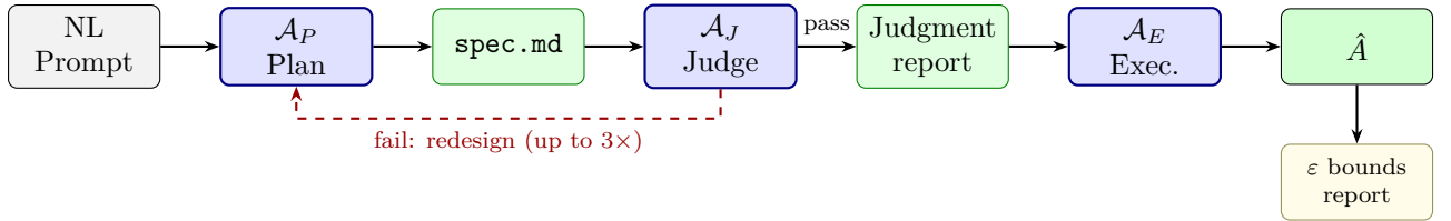
Figure 1. Specification-driven design pipeline. A natural-language prompt is the sole user input. \mathcal{A}_P generates a spec.md ; \mathcal{A}_J validates in three stages: (1) structural compilation, (2) Triad gate evaluation [3], (3) cost and feasibility assessment (see Figure 6 for details). Failed designs are fed back with a redesign prompt (dashed red, up to 3 rounds). \mathcal{A}_E executes reconstruction and outputs \hat{A} with an explicit \varepsilon -bound report. See Figure 3 for per-modality error breakdown.
