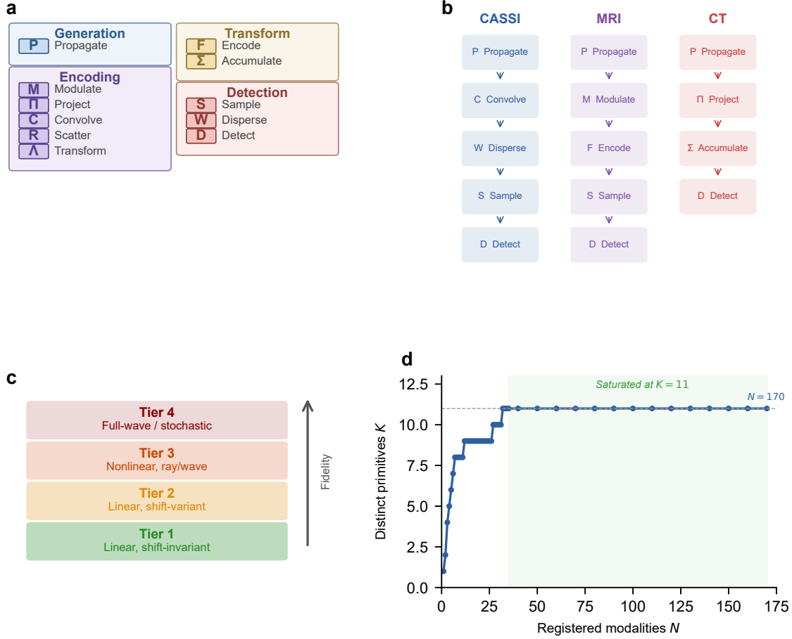
Figure 2: 11 primitives: OperatorGraph IR, Physics Fidelity Ladder, and basis completeness. a , The 11 universal primitives grouped by physical role: generation (Propagate P ), encoding (Modulate M , Project \Pi , Convolve C , Scatter R , Transform \Lambda ), transform (Encode F , Accumulate \Sigma ), and detection (Sample S , Disperse W , Detect D ). Each primitive carries a typed signature mapping its input to its output (e.g., P : free-space propagation; D : detector response). b , Example OPERATORGRAPH DAGs for three modalities: CASSI (photon), MRI (spin), and CT (X-ray photon). Each node wraps a primitive operator; edges define data flow. The symbols in panel b correspond directly to the primitive labels in panel a. c , Fidelity levels: forward models range from linear shift-invariant (simplest) through nonlinear and full-wave; all 11 primitives apply uniformly across every level. d , Basis-growth saturation: the number of distinct primitives K required to express N registered modalities saturates at K=11 for N \geq 35 ; no additional primitive has been needed for the 135 subsequent modalities across 23 physical categories.
