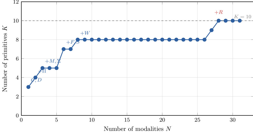
Figure 1: Basis-growth saturation. Number of distinct primitives K as a function of the number of modalities N added to the registry. The curve saturates at K = 10 for N \geq 28 ; annotated points mark each primitive introduction. Saturation is consistent with Theorem 18: once all physics-stage families are covered, new modalities compose existing primitives.
