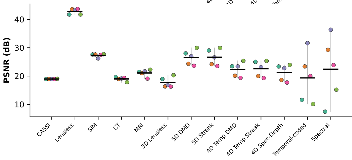
(b) PSNR spread per modality (5 algorithms each)
